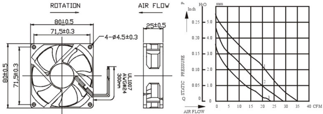
BRUSHLESS FAN 80 × 80 × 25mm
